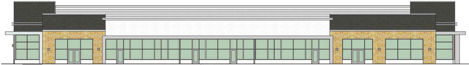
BUILDING ELEVATION
